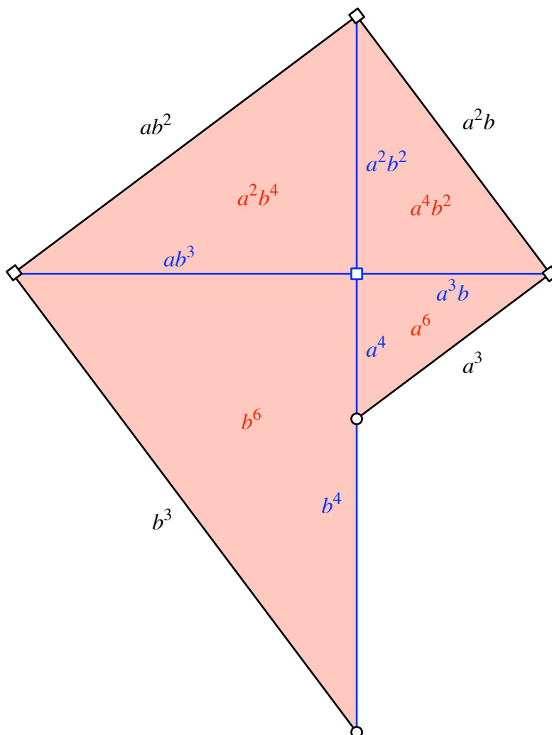
Abb. 2: Iteration
